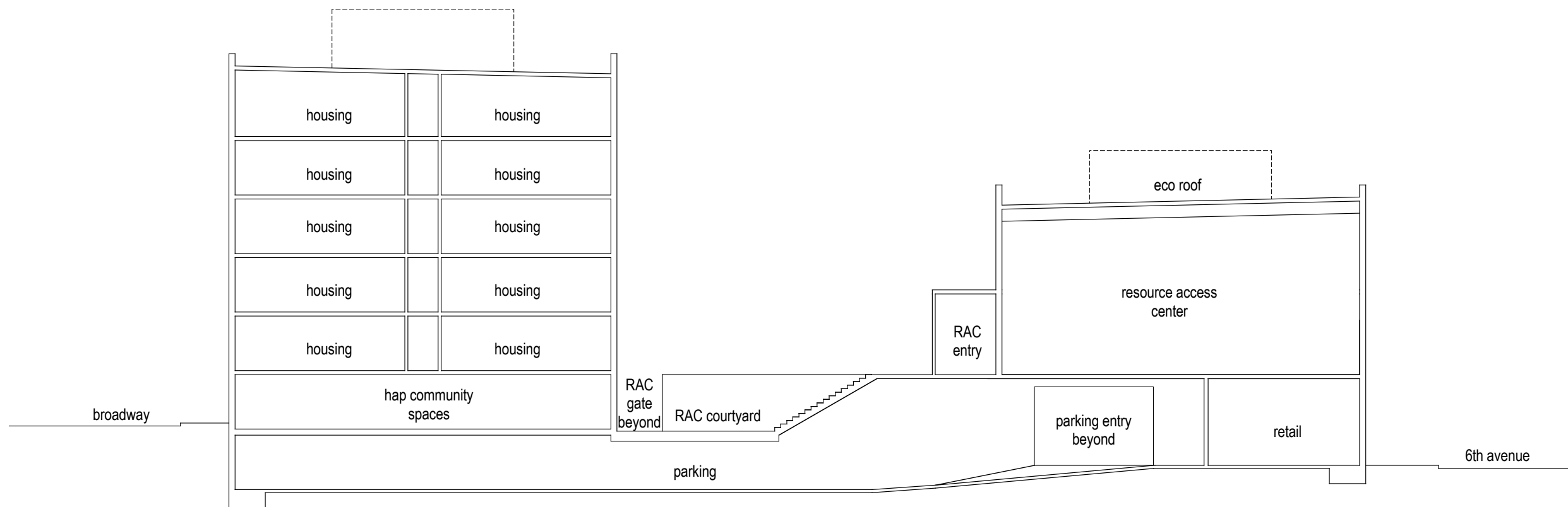
Housing on Broadway Scheme section looking north
