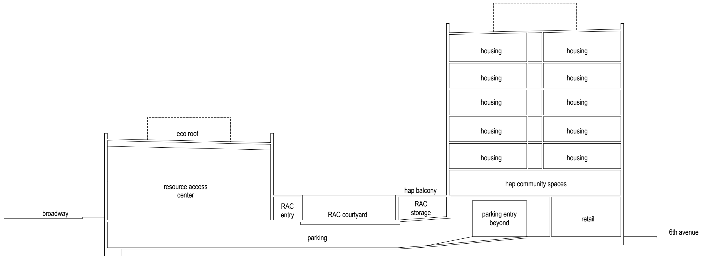
Housing on 6th Avenue Scheme section looking north
